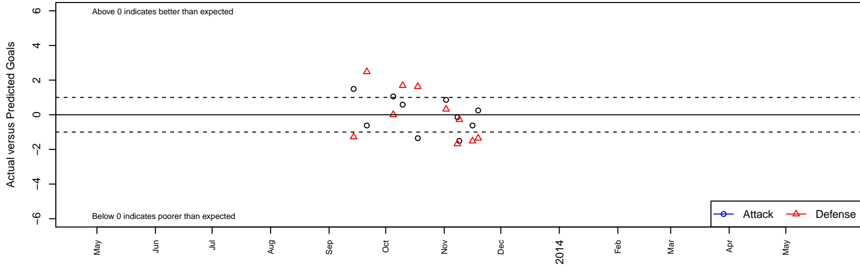
Woodland Fire G01 Dots are actual minus expected GF (blue circles) and GA (red triangles). Blue line is smoothed change in attack strength. Red is smoothed change in defense strength.
